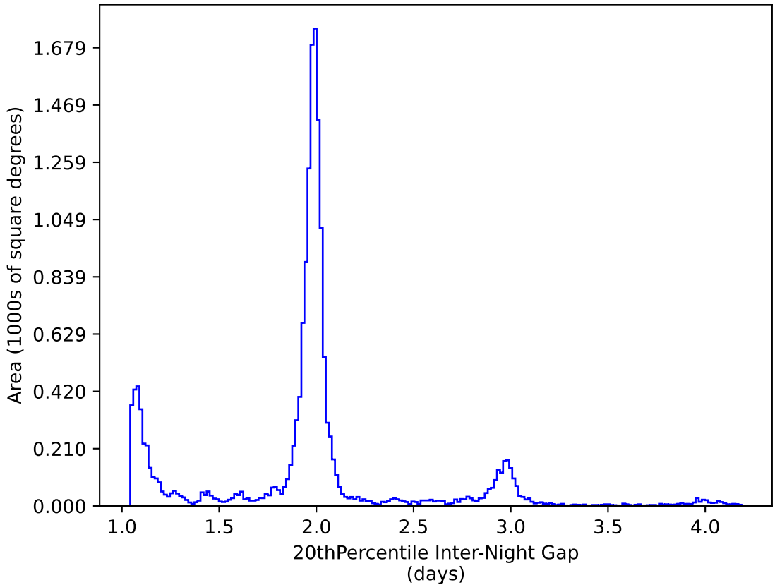
ddf_acor_sf30_lsf40_lsr10_v3.4_10yrs WFD y band: 20thPercentile Inter-Night Gap
