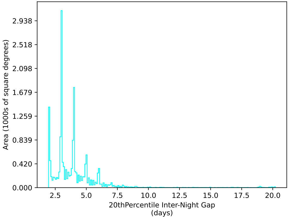
ddf_acor_sf30_ls40_lsr10_v3.4_10yrs WFD u band: 20thPercentile Inter-Night Gap
