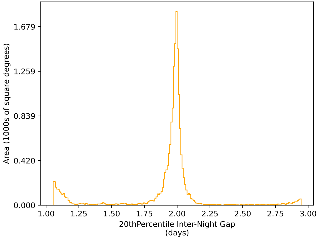
ddf_acor_sf30_lsf40_lsr10_v3.4_10yrs WFD r band: 20thPercentile Inter-Night Gap
