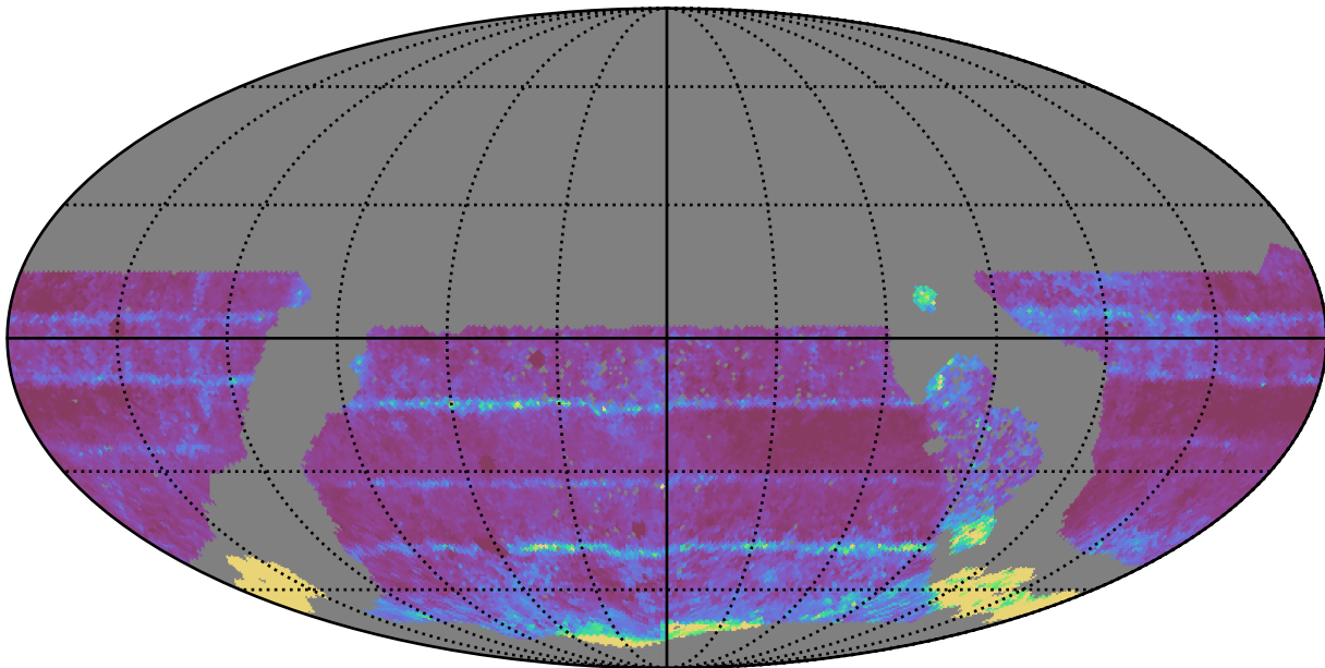
ddf_acor_sf30_lsf40_lsr10_v3.4_10yrs WFD all bands: 20thPercentile Inter-Night Gap
