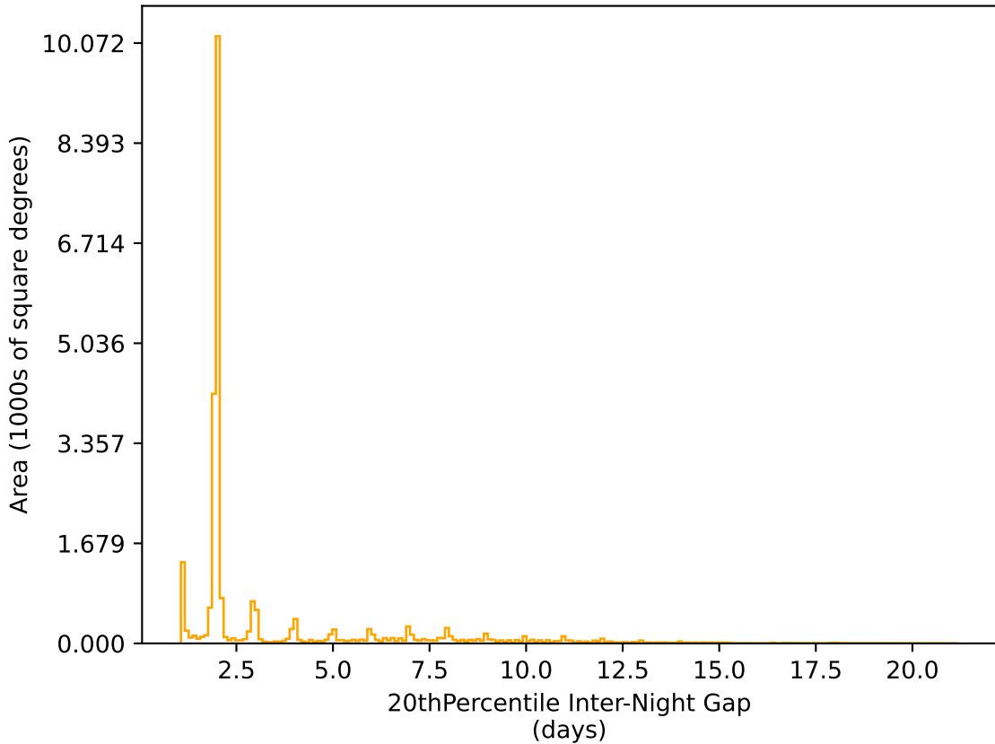
ddf_acor_sf30_lsf40_lsr10_v3.4_10yrs All sky r band: 20thPercentile Inter-Night Gap
