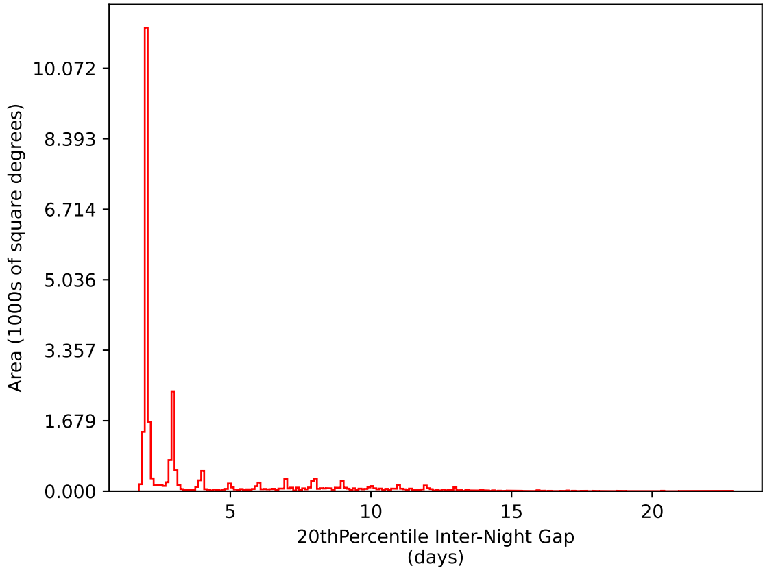
ddf_acor_sf30_ls40_lsr10_v3.4_10yrs All sky i band: 20thPercentile Inter-Night Gap
