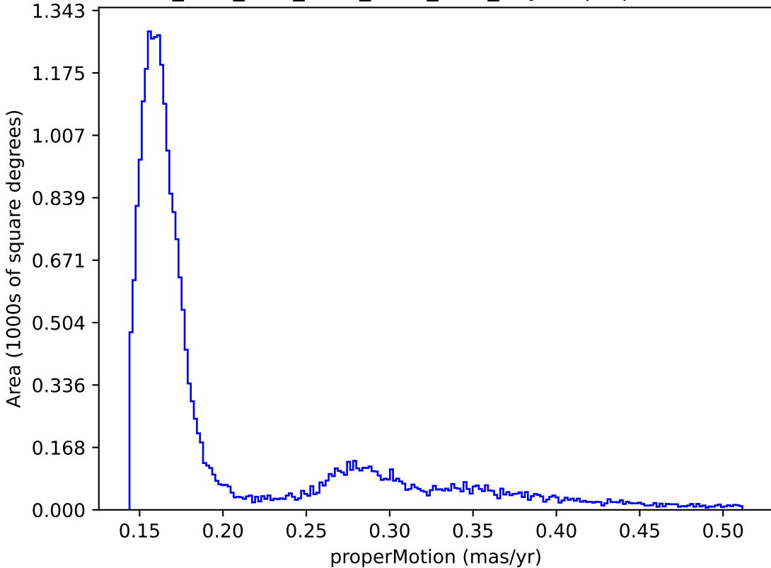
ddf_acor_sf30_lsf40_lsr10_v3.4_10yrs : properMotion
