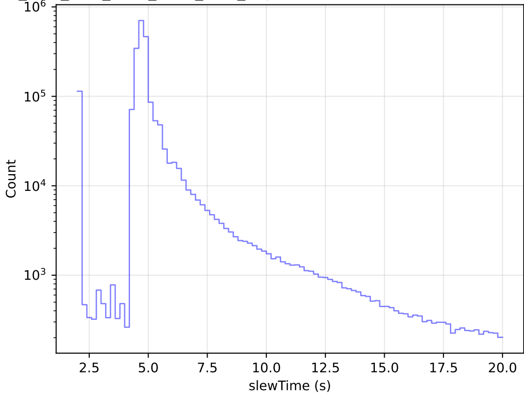
ddf_acor_sf30_Isf40_Isr10_v3.4_10yrs All visits: Zoom Slew Time Histogram
