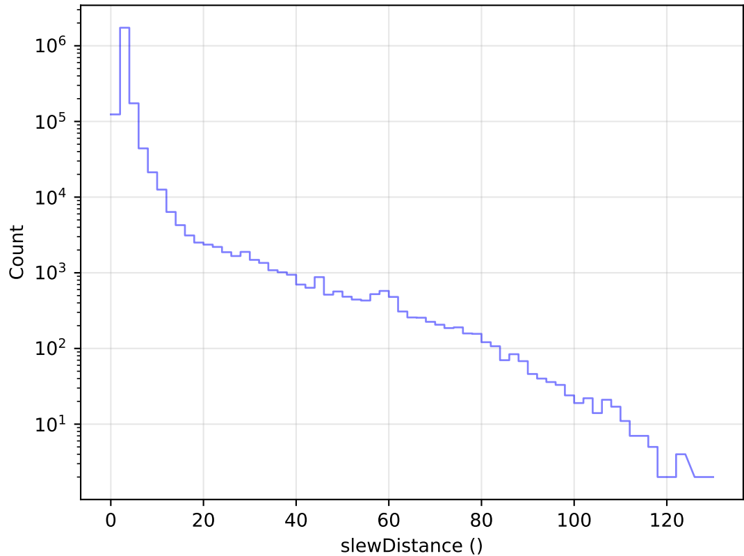
ddf_acor_sf30_lsf40_lsr10_v3.4_10yrs All visits: Slew Distance Histogram
