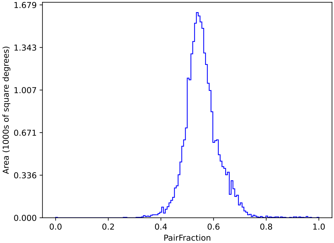
ddf_acor_sf30_lsf40_lsr10_v3.4_10yrs (g or r or i): PairFraction
