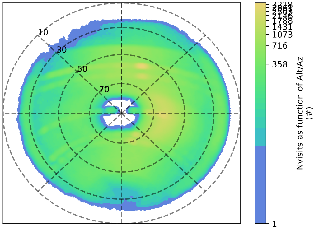
ddf_acor_sf30_lsf40_lsr10_v3.4_10yrs z: Nvisits as function of Alt/Az
