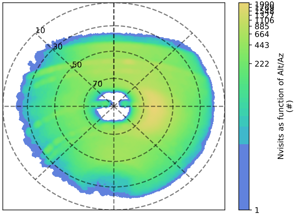
ddf_acor_sf30_lsf40_lsr10_v3.4_10yrs y: Nvisits as function of Alt/Az
