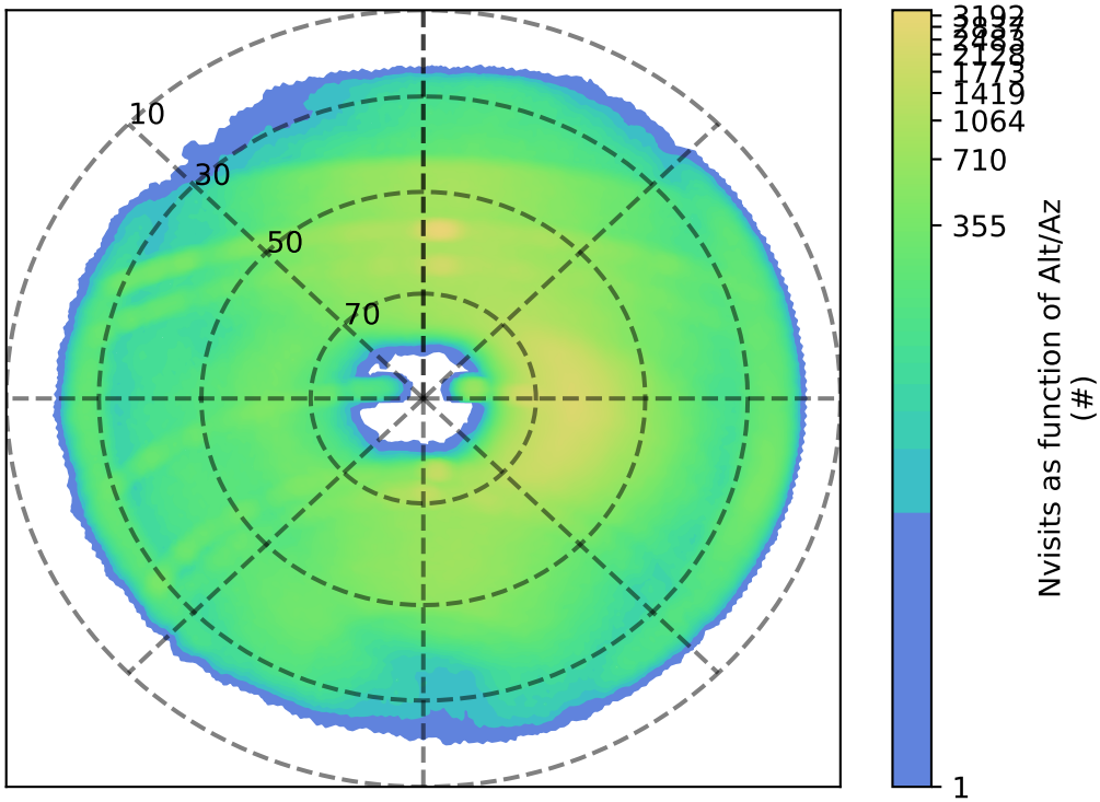
ddf_acor_sf30_lsf40_lsr10_v3.4_10yrs i: Nvisits as function of Alt/Az
