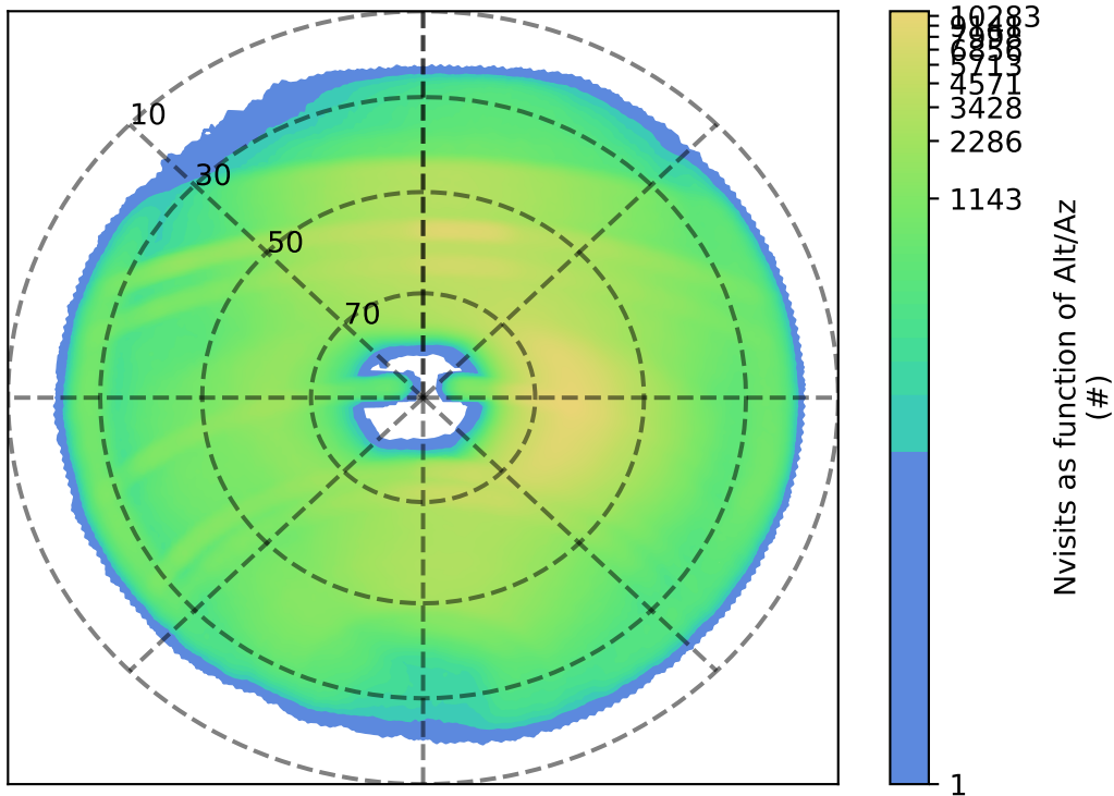
ddf_acor_sf30_lsf40_lsr10_v3.4_10yrs : Nvisits as function of Alt/Az
