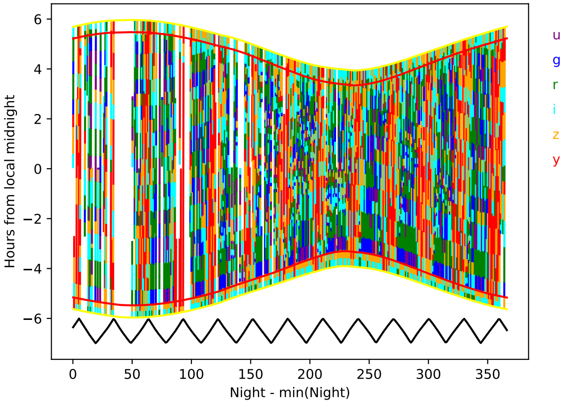
ddf_acor_sf30_lsf40_lsr10_v3.4_10yrs year 6-7: Hourglass
