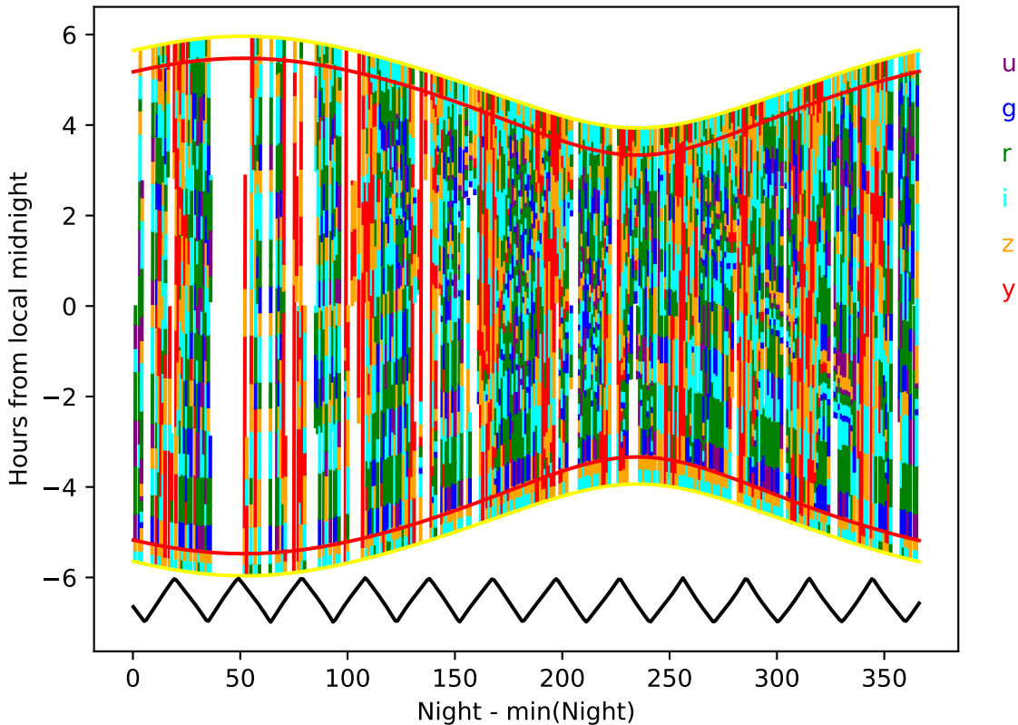
ddf_acor_sf30_lsf40_lsr10_v3.4_10yrs year 2-3: Hourglass
