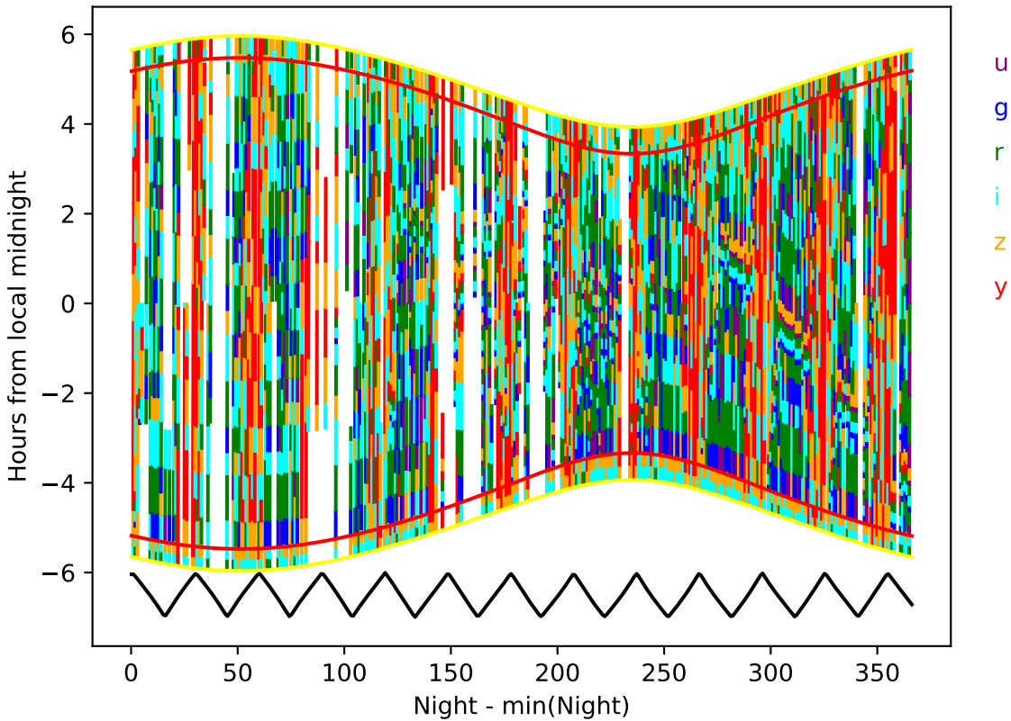
ddf_acor_sf30_lsf40_lsr10_v3.4_10yrs year 1-2: Hourglass
