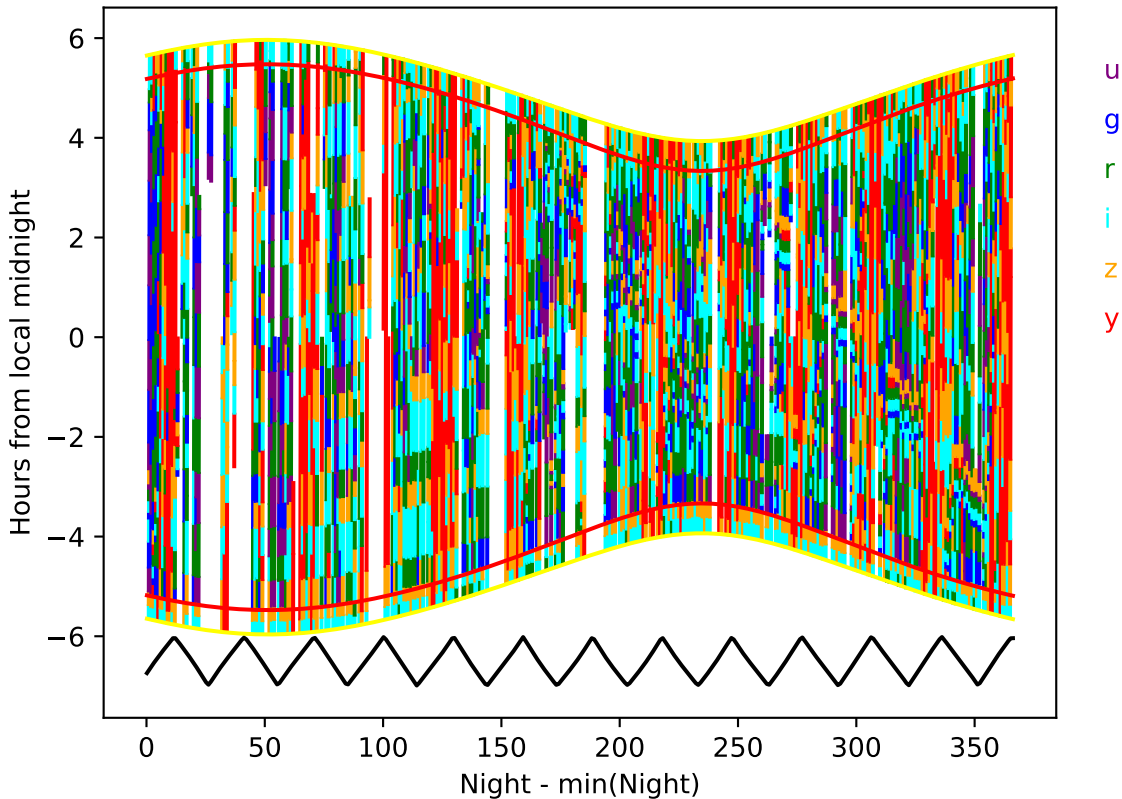
ddf_acor_sf30_lsf40_lsr10_v3.4_10yrs year 0-1: Hourglass
