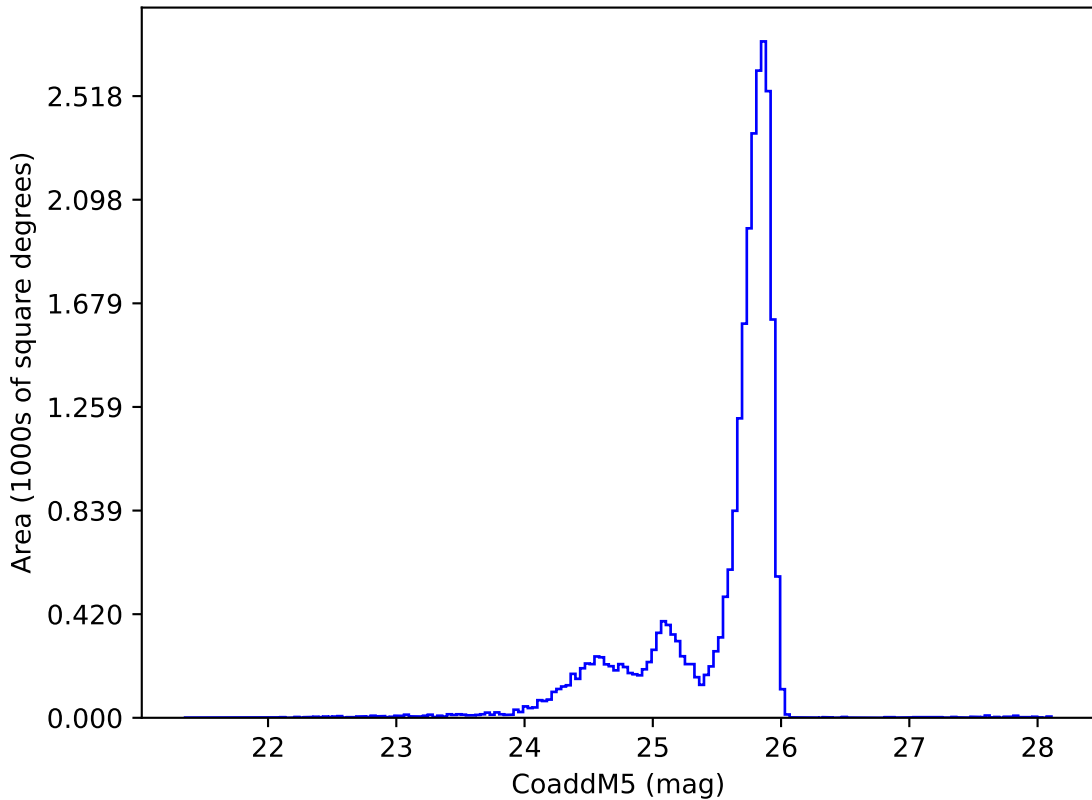
ddf_acor_sf30_lsf40_lsr10_v3.4_10yrs z: CoaddM5
