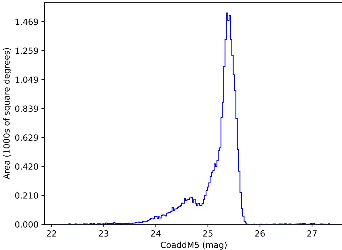
ddf_acor_sf30_lsf40_lsr10_v3.4_10yrs u: CoaddM5
