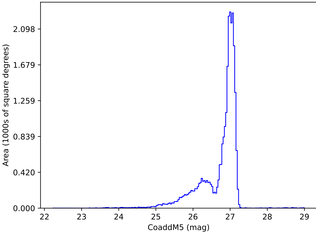
ddf_acor_sf30_lsf40_lsr10_v3.4_10yrs r: CoaddM5
