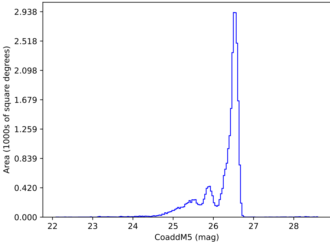
ddf_acor_sf30_lsf40_lsr10_v3.4_10yrs i: CoaddM5
