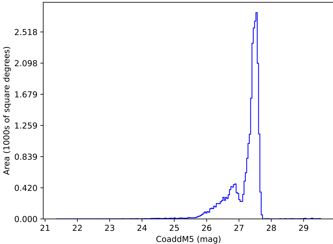
ddf_acor_sf30_lsf40_lsr10_v3.4_10yrs : CoaddM5
