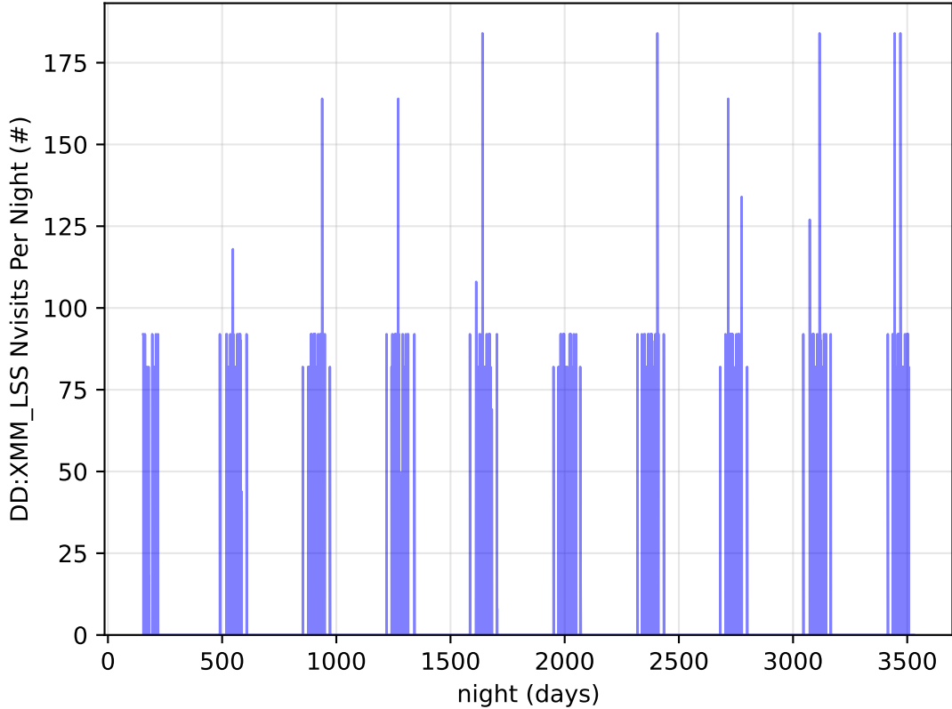
ddf_acor_sf30_lsf40_lsr10_v3.4_10yrs all bands: DD:XMM_LSS Nvisits Per Night
