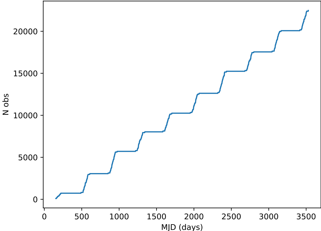
ddf_acor_sf30_lsf40_lsr10_v3.4_10yrs all bands: DD:XMM_LSS Cumulative NVisits
