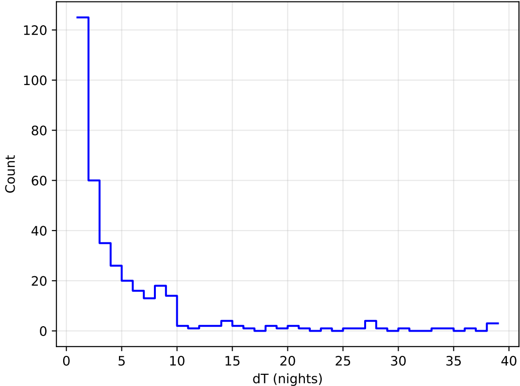
ddf_acor_sf30_lsf40_lsr10_v3.4_10yrs all bands: DD:WFD Delta Nights Histogram
