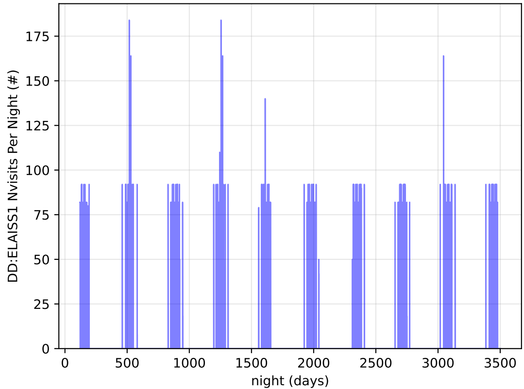
ddf_acor_sf30_lsf40_lsr10_v3.4_10yrs all bands: DD:ELAISS1 Nvisits Per Night
