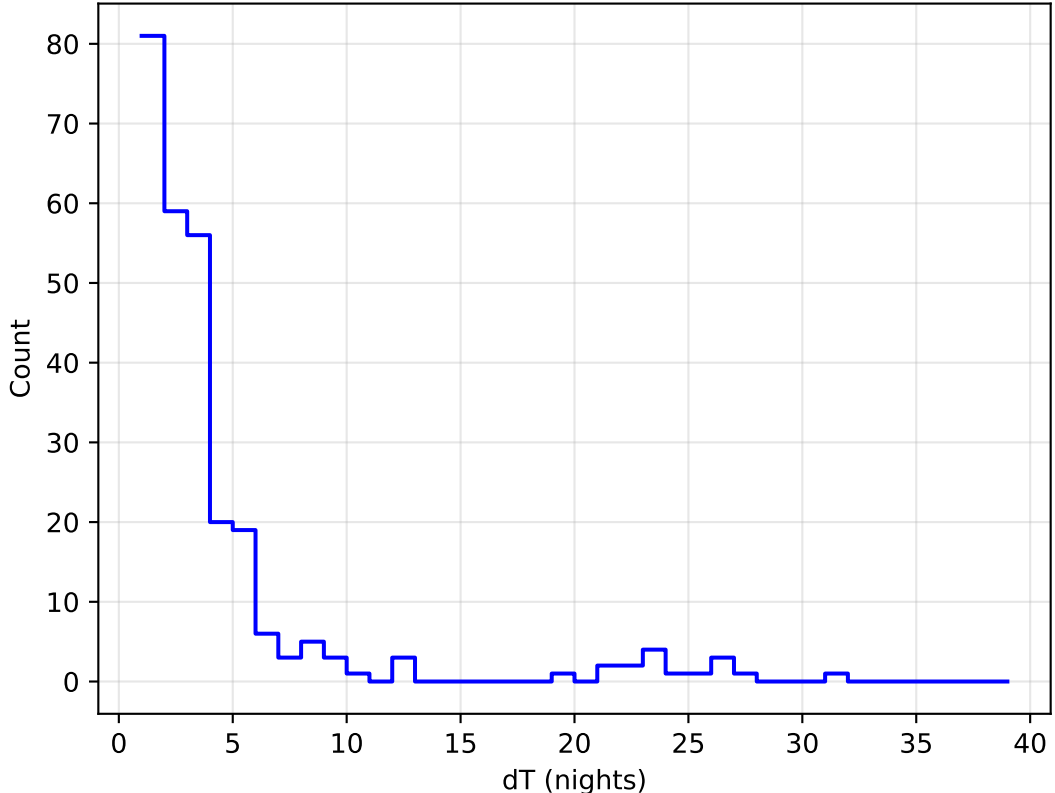
ddf_acor_sf30_lsf40_lsr10_v3.4_10yrs all bands: DD:ELAISS1 Delta Nights Histogram
