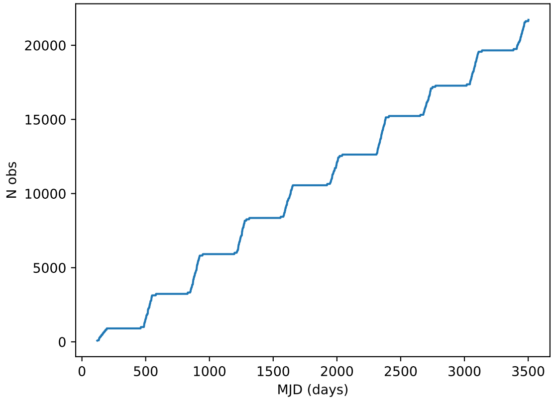
ddf_acor_sf30_Isf40_Isr10_v3.4_10yrs all bands: DD:ELAISS1 Cumulative NVisits
