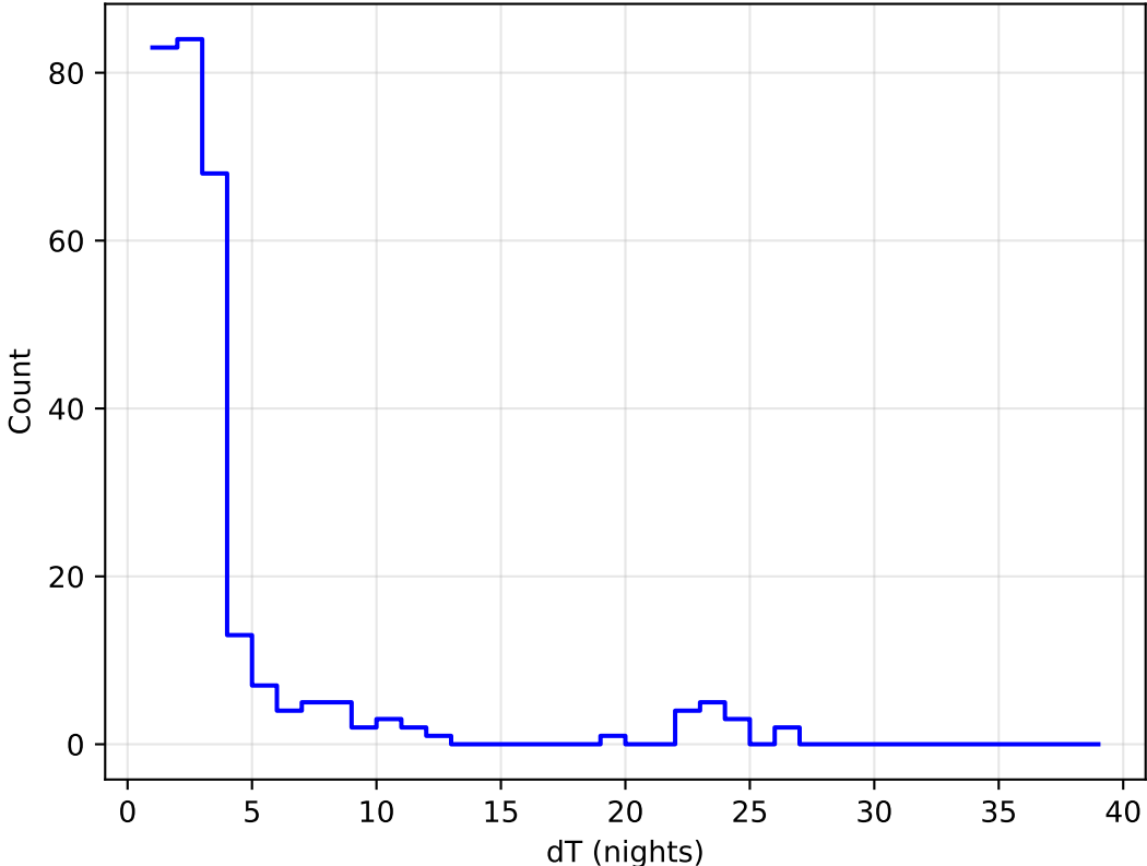
ddf_acor_sf30_Isf40_Isr10_v3.4_10yrs all bands: DD:EDFS Delta Nights Histogram
