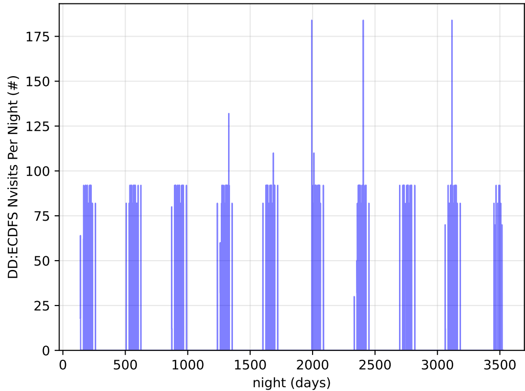
ddf_acor_sf30_lsf40_lsr10_v3.4_10yrs all bands: DD:ECDFS Nvisits Per Night
