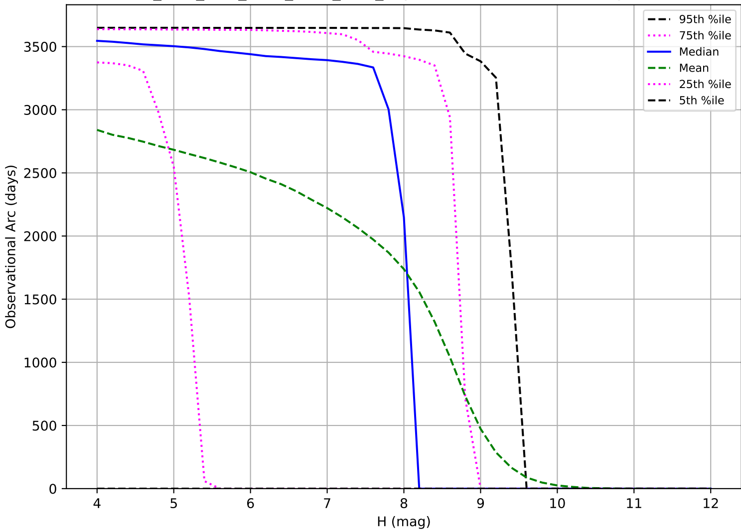
ddf_acor_sf25_Isf40_Isr50_v3.4_10yrs: Observational Arc Length TNO
