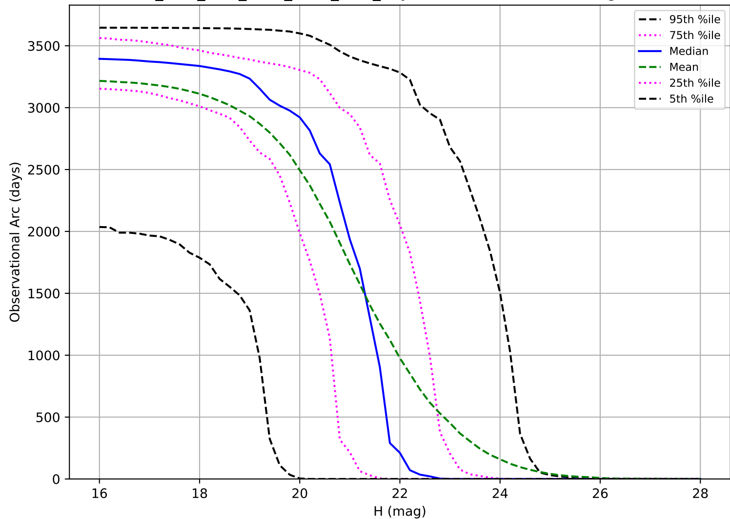
ddf_acor_sf25_lsf40_lsr50_v3.4_10yrs: Observational Arc Length PHA
