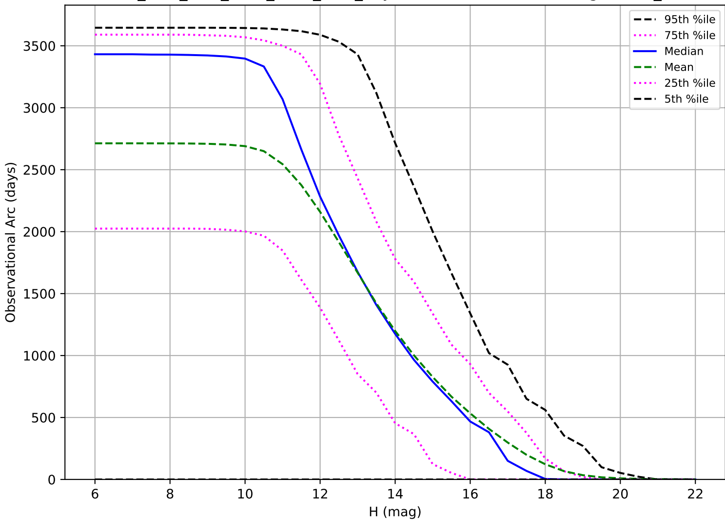
ddf_acor_sf25_lsf40_lsr50_v3.4_10yrs: Observational Arc Length OCC_r5
