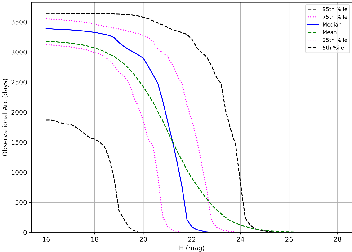
ddf_acor_sf25_lsf40_lsr50_v3.4_10yrs: Observational Arc Length NEO
