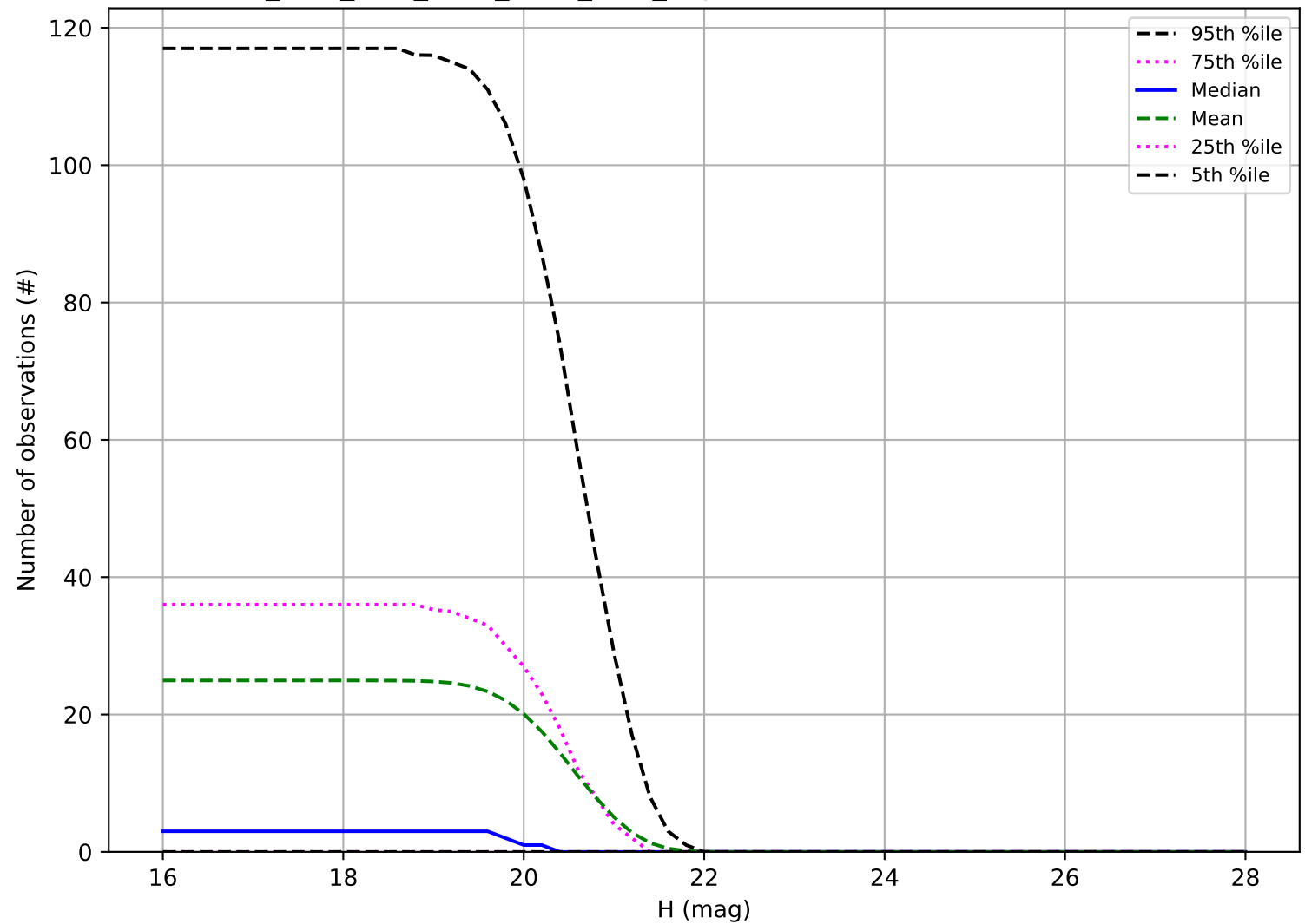
ddf_acor_sf25_lsf40_lsr50_v3.4_10yrs: Number of observations Vatira
