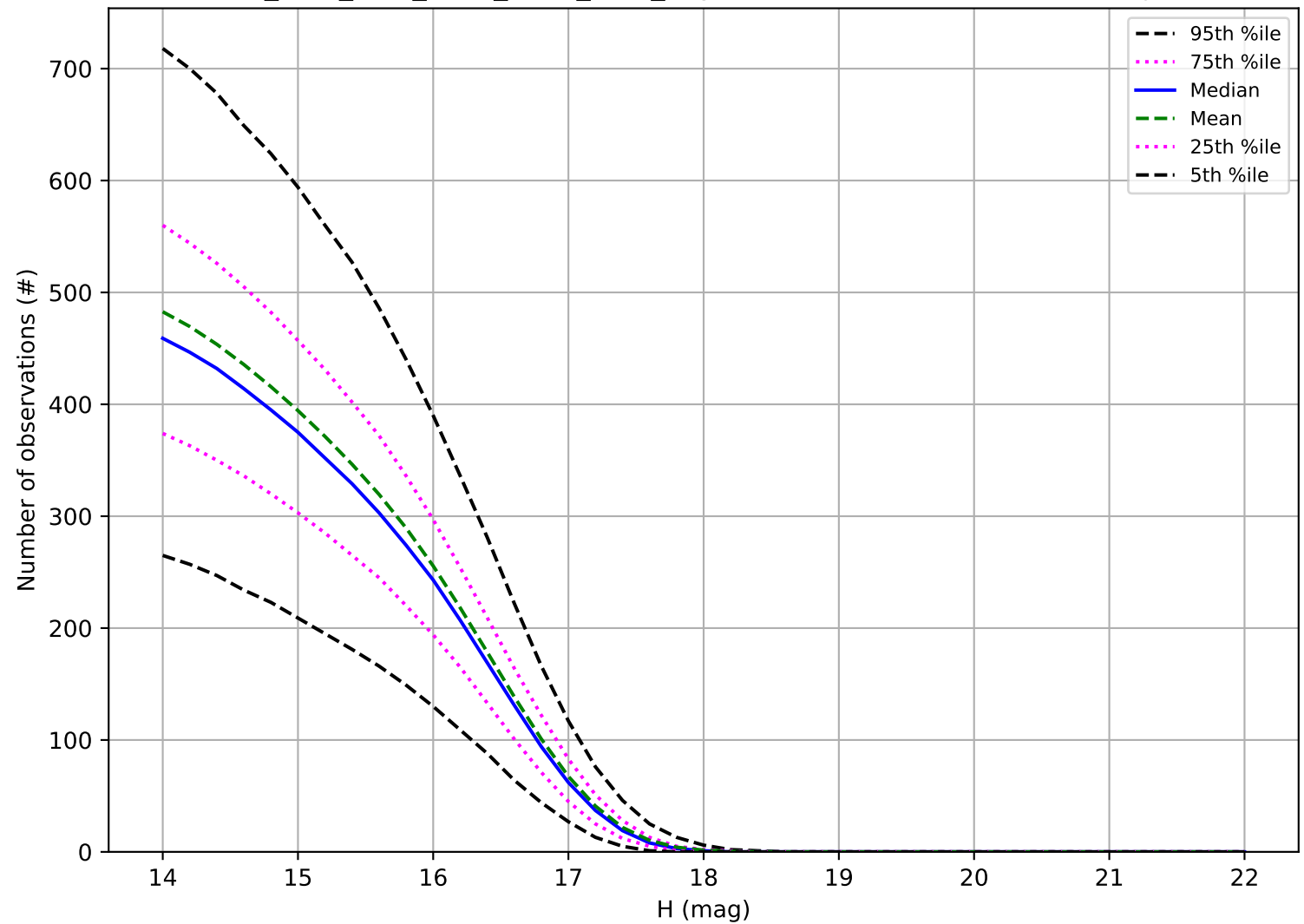
ddf_acor_sf25_lsf40_lsr50_v3.4_10yrs: Number of observations Trojan
