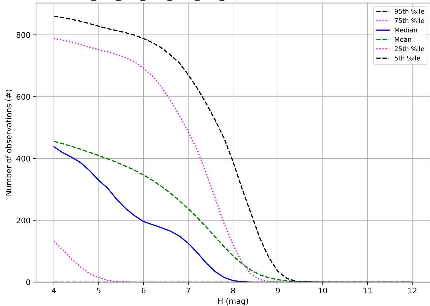
ddf_acor_sf25_lsf40_lsr50_v3.4_10yrs: Number of observations TNO
