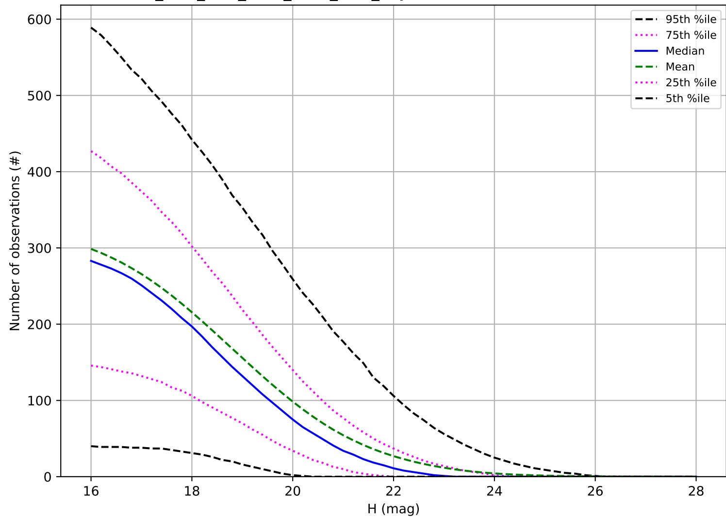
ddf_acor_sf25_lsf40_lsr50_v3.4_10yrs: Number of observations PHA
