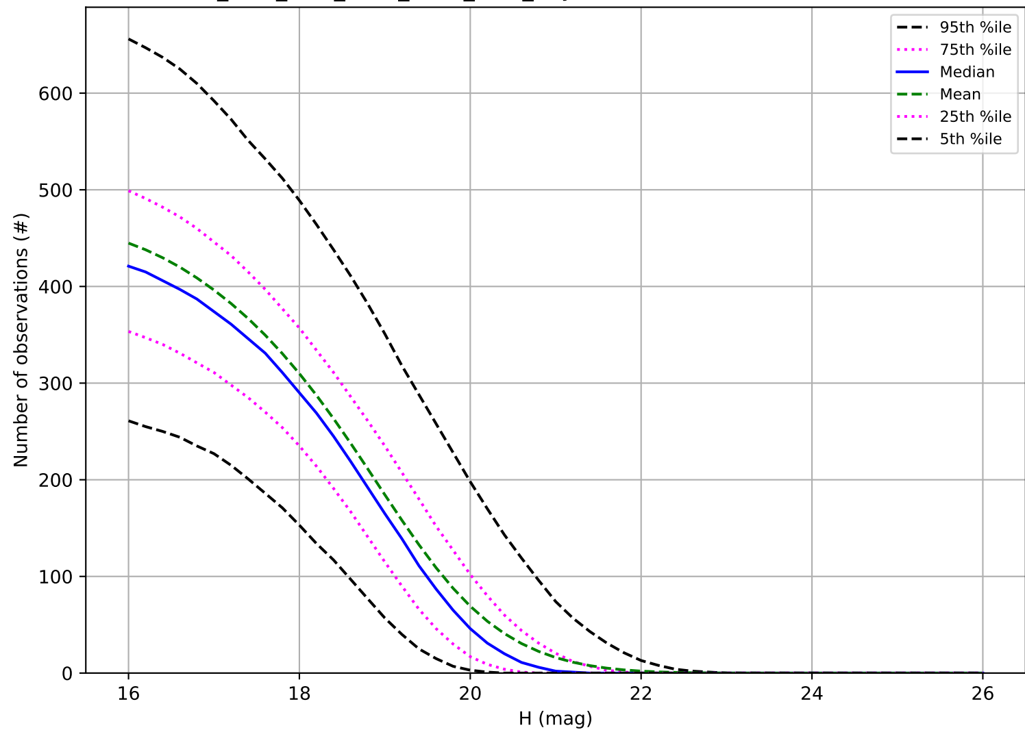
ddf_acor_sf25_Isf40_Isr50_v3.4_10yrs: Number of observations MBA
