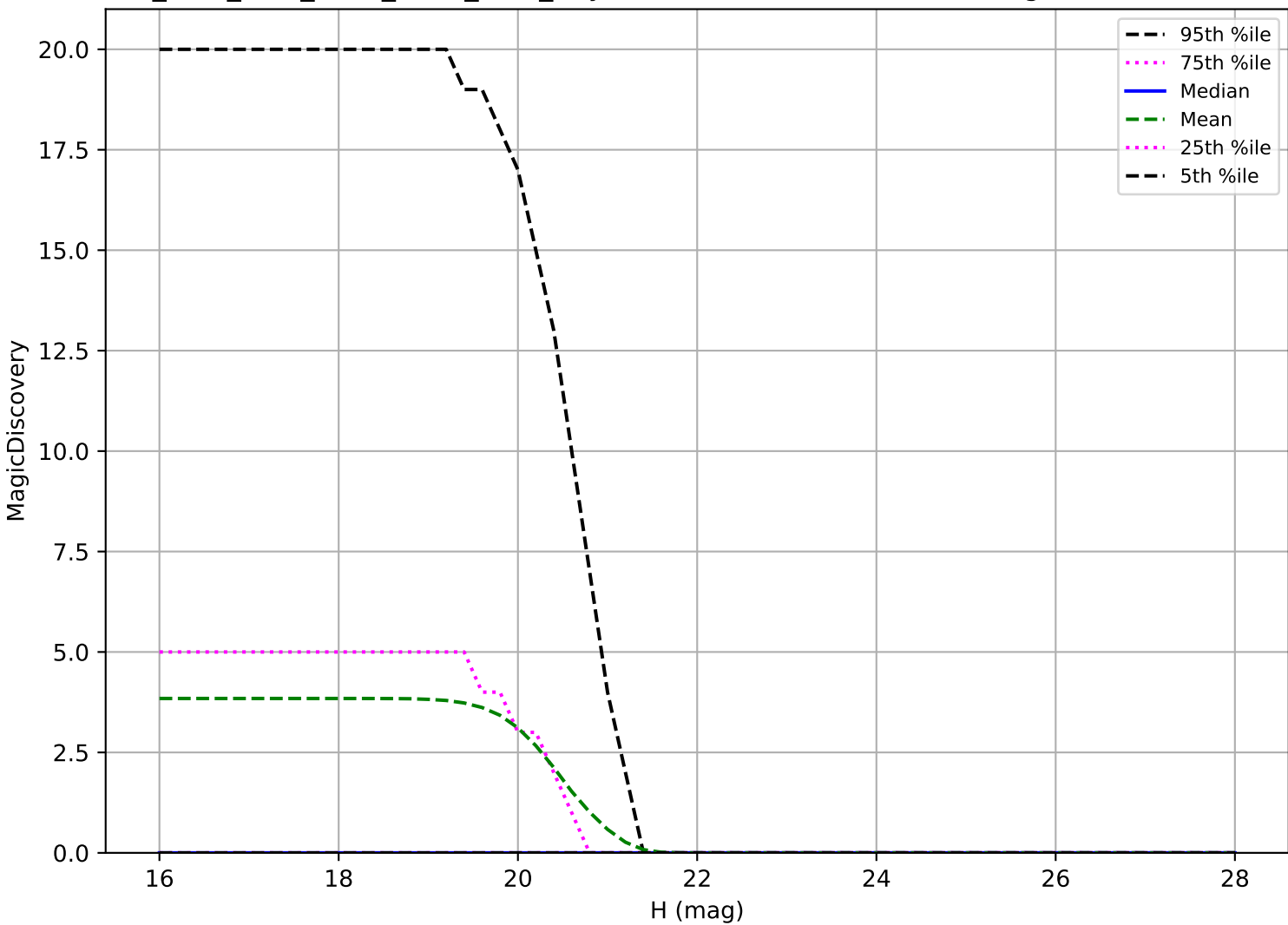
ddf_acor_sf25_lsf40_lsr50_v3.4_10yrs: Vatra 6 detections in 60 nights detection loss
