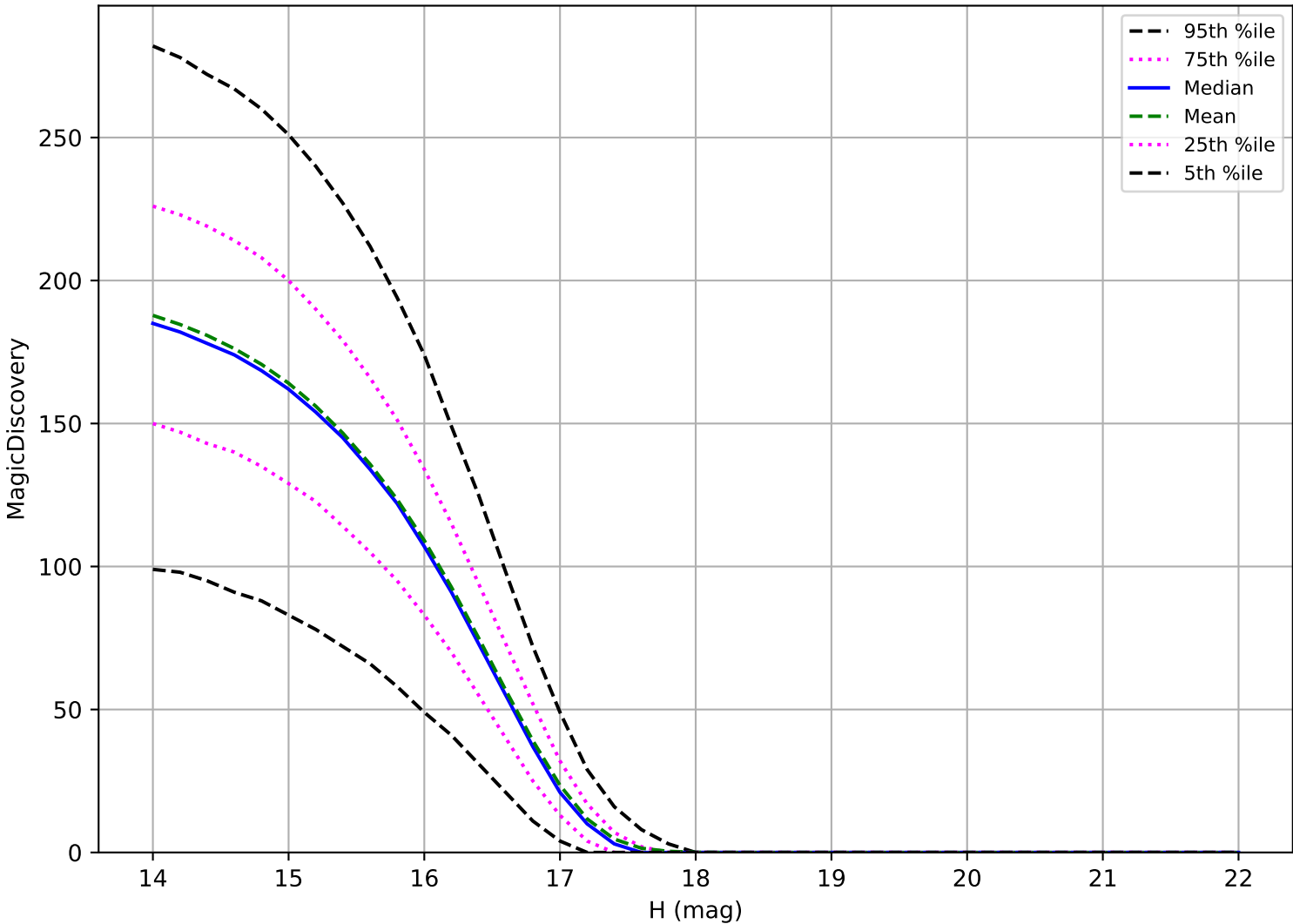
ddf_acor_sf25_lsf40_lsr50_v3.4_10yrs: Trojan 6 detections in 60 nights detection loss
