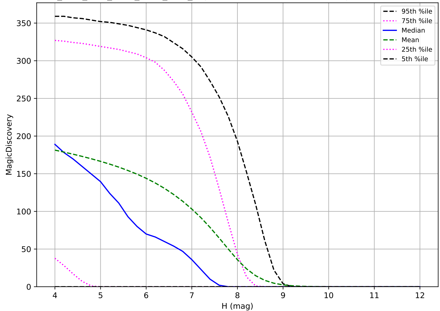
ddf_acor_sf25_lsf40_lsr50_v3.4_10yrs: TNO 6 detections in 60 nights detection loss
