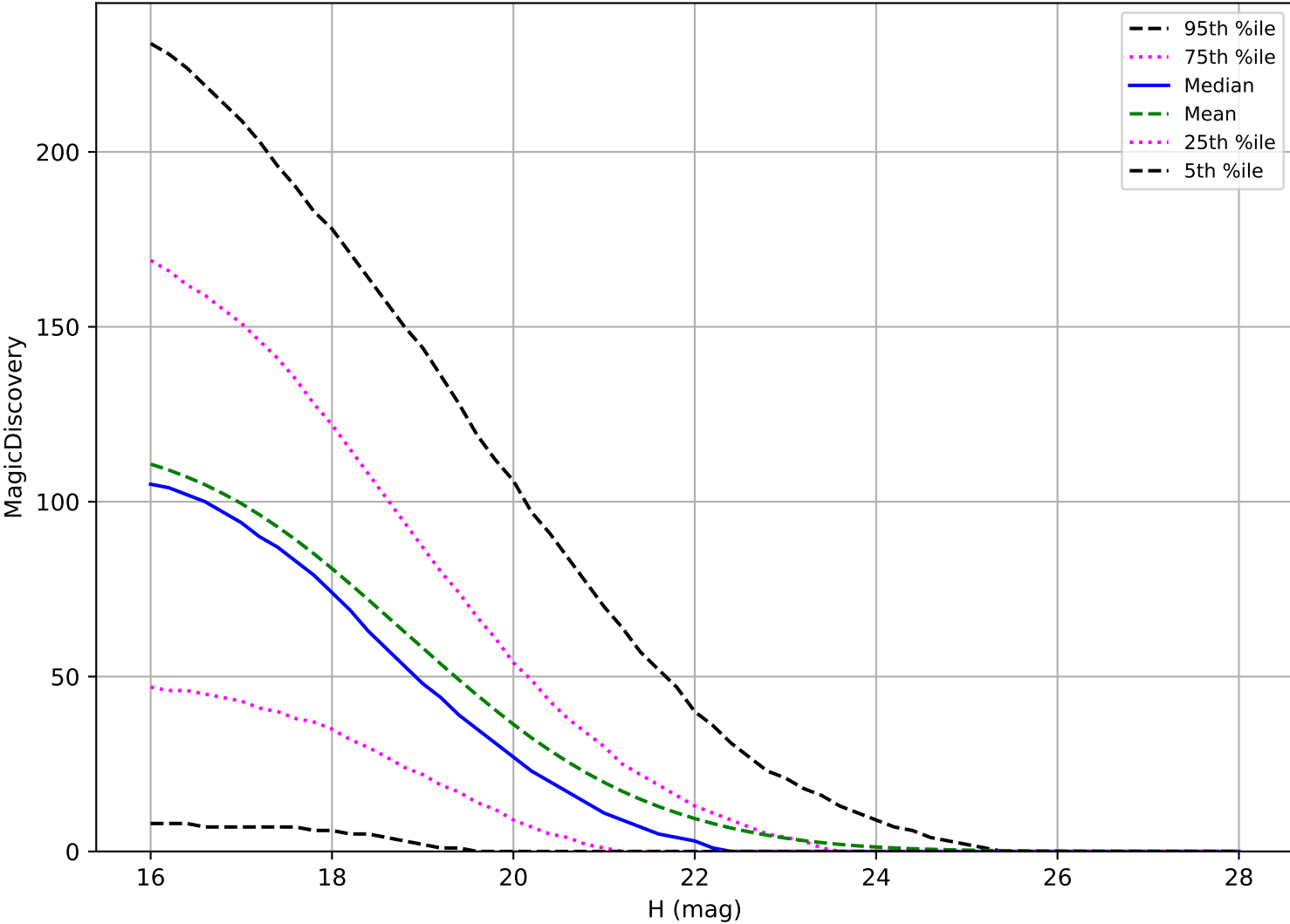
ddf_acor_sf25_lsf40_lsr50_v3.4_10yrs: PHA 6 detections in 60 nights detection loss
