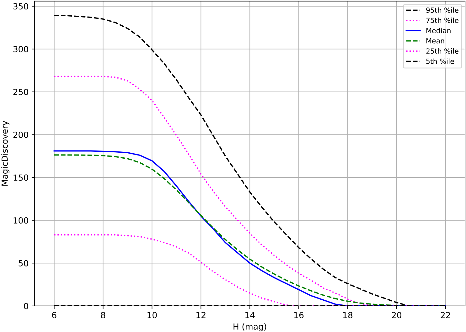
ddf_acor_sf25_lsf40_lsr50_v3.4_10yrs: OCC_r5 6 detections in 60 nights detection loss
