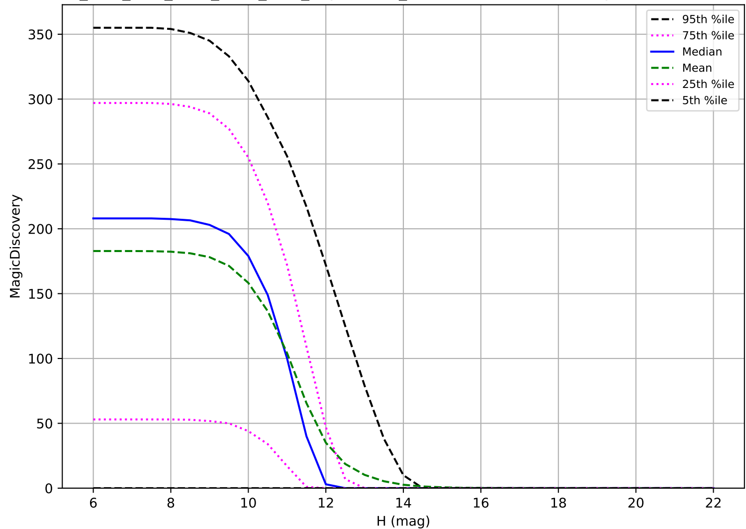
ddf_acor_sf25_lsf40_lsr50_v3.4_10yrs: OCC_r20 6 detections in 60 nights detection loss
