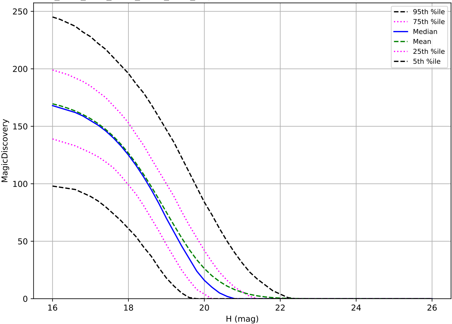
ddf_acor_sf25_lsf40_lsr50_v3.4_10yrs: MBA 6 detections in 60 nights detection loss
