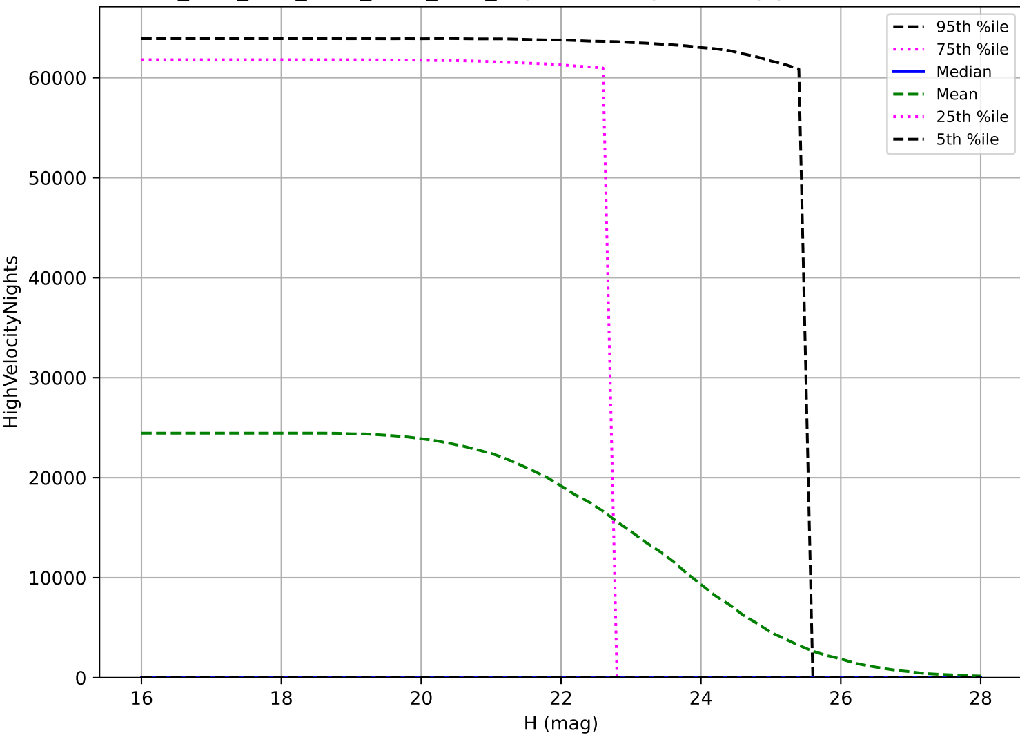
ddf_acor_sf25_lsf40_lsr50_v3.4_10yrs: PHA High velocity pair detection loss
