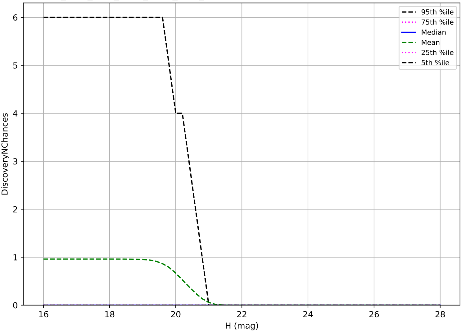
ddf_acor_sf25_lsf40_lsr50_v3.4_10yrs: Vatira 3 pairs in 15 nights detection loss
