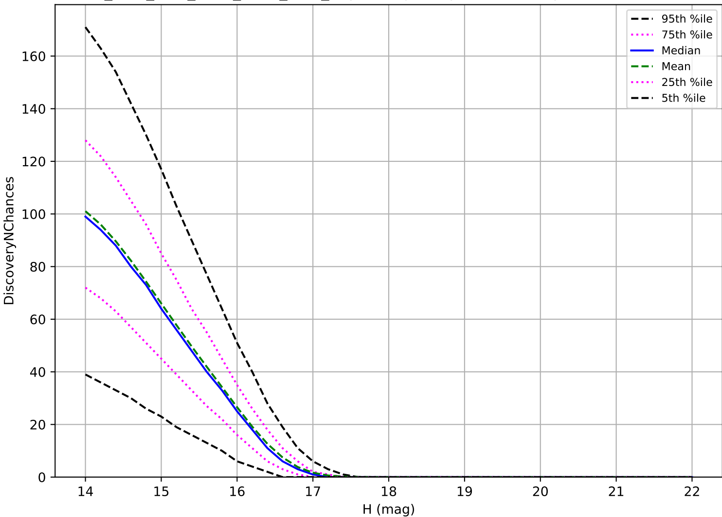
ddf_acor_sf25_lsf40_lsr50_v3.4_10yrs: Trojan 3 pairs in 15 nights detection loss
